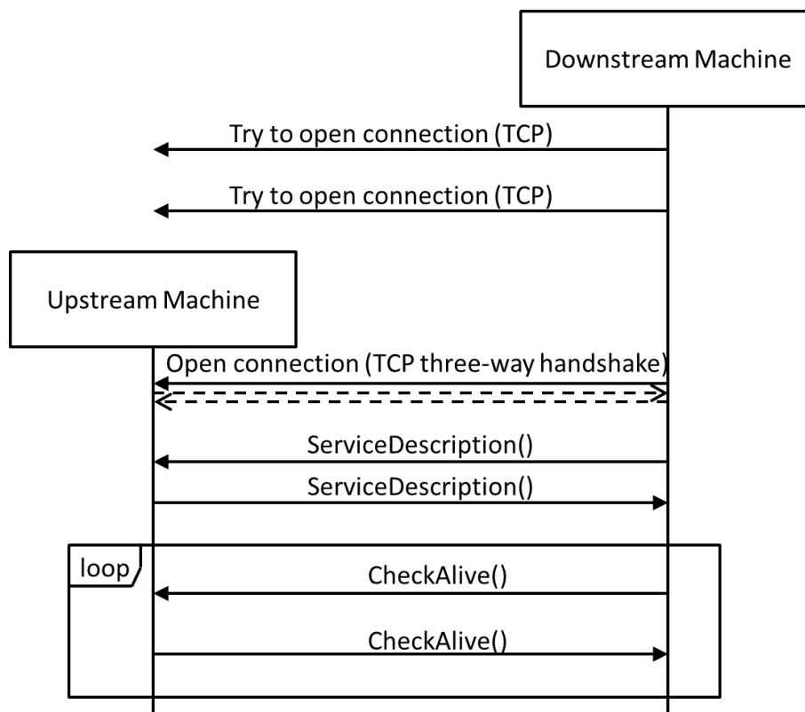
Fig. 1 Connection, handshake and connection loss detection
